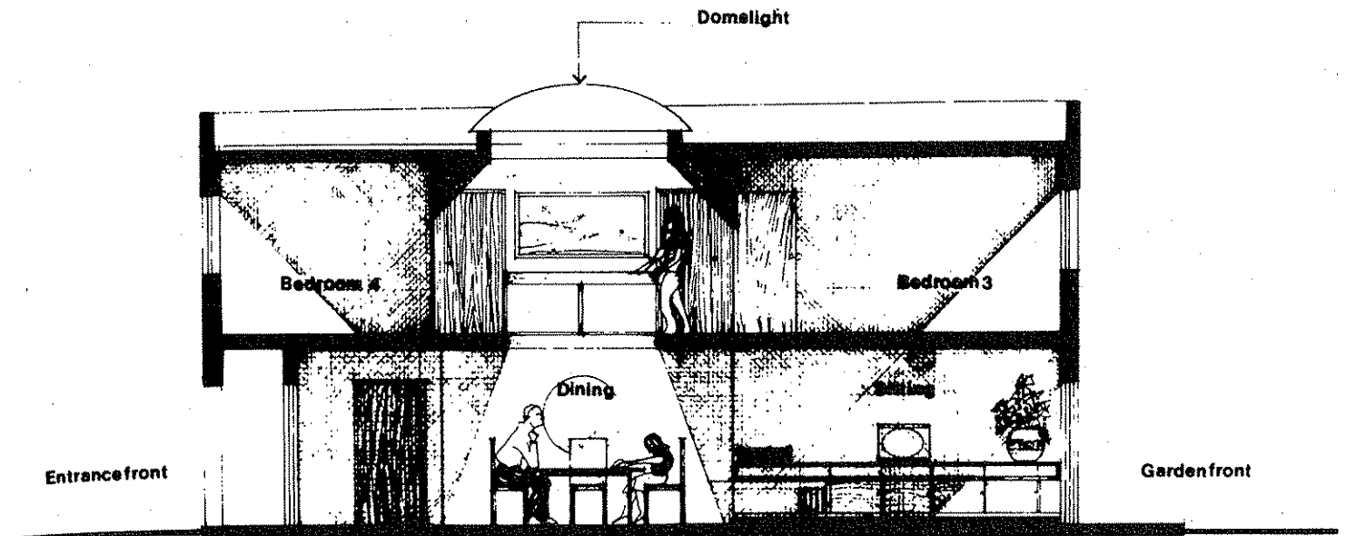
Section AA
